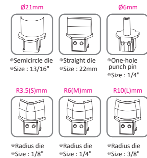
Calibration device
